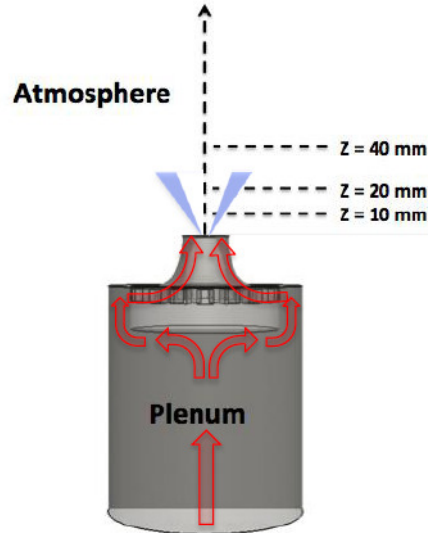
Fig. 2 Experimental setup. Air path in red, spray injection in blue. From [6].
