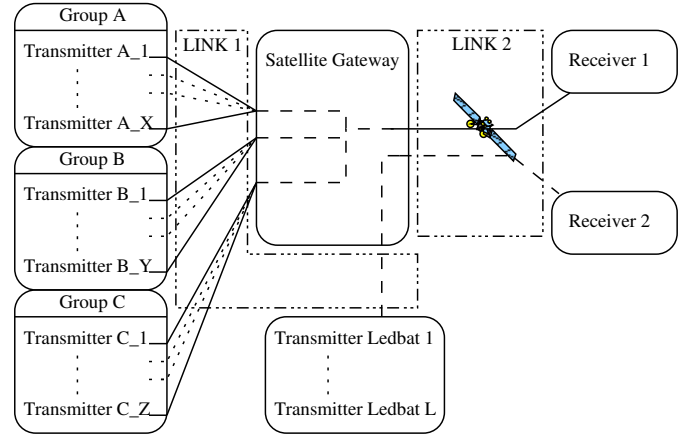
Fig. 1. Network architecture
