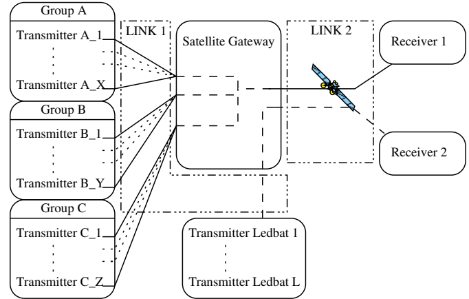
Fig. 1. Network architecture
