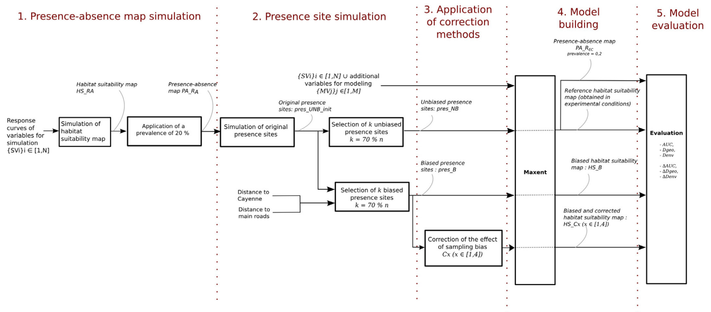
Fig. 2. Overall processing chain for data simulation, bias application, and the subsequent application, evaluation, and comparison of the correction methods in the framework of Maxent modeling.
