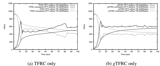
Figure 10. Over-provisioned network
