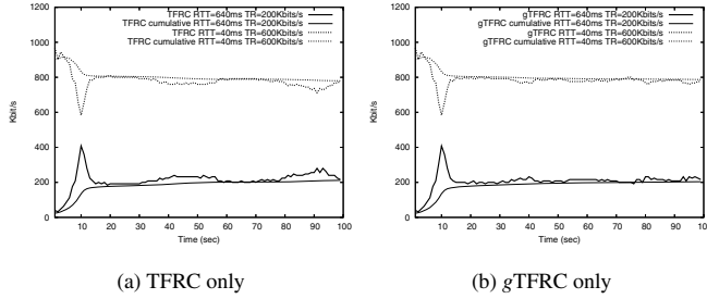
Figure 11. Over-provisioned network
