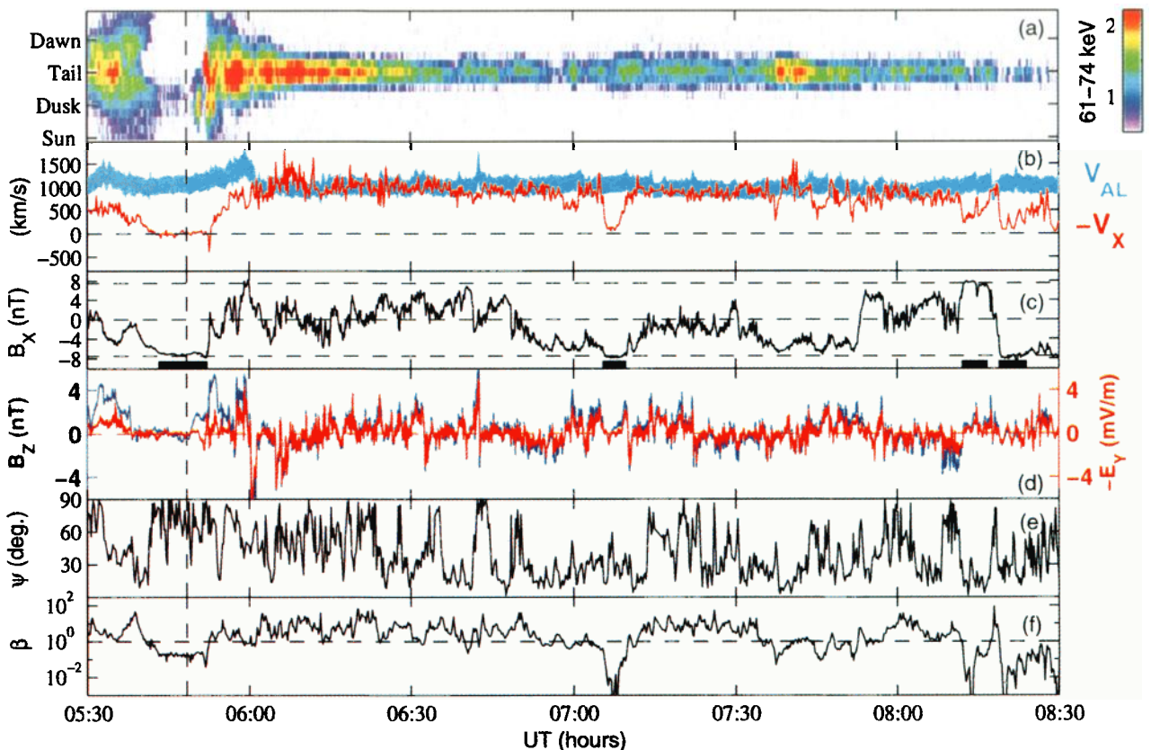
Figure 2. Three hours of data obtained onboard GEOTAIL. Panel (a): Angular distribution of 61-74 keV ions in the equatorial [X-Y]GSE plane. The color scale gives the log of differential flux. The labels of the Y-axis designate the direction of the particles; (b): tailward component of the plasma bulk velocity (red line) and lobe Alfvén velocity range (blue shadowed area); (c): B_x component of the magnetic field; (d): B_z component of the magnetic field (left axis) and -E_y component of the electric field (right axis); (e): Variation of the angle \psi (see text); Panel (f): \beta plasma parameter.
