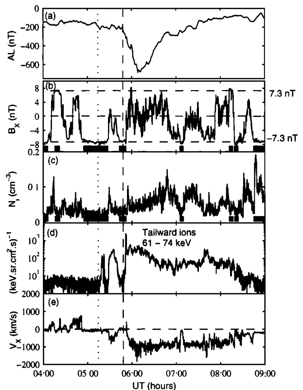
Figure 1. Five hours of data obtained on the ground and at GEOTAIL orbit ( X_{GSE} = -133R_E ). Panel (a): 1 minute AL index variations. The onset of the substorm is represented by the vertical dashed line; (b): B_x component of the magnetic field; (c): Ion number density. The shadowed area is drawn for density values between 0.02 and 0.04 \text{cm}^{-3} ; (d): Differential flux of 61-74 keV tailward ions; (e): V_x component of the plasma bulk velocity. The black areas at the bottom of panels (b) and (c) represent periods when GEOTAIL was located in the lobes, defined by B_x \sim 7.3 nT. The dashed (dotted) vertical line indicates the substorm onset time (moderate electrojet activation).
