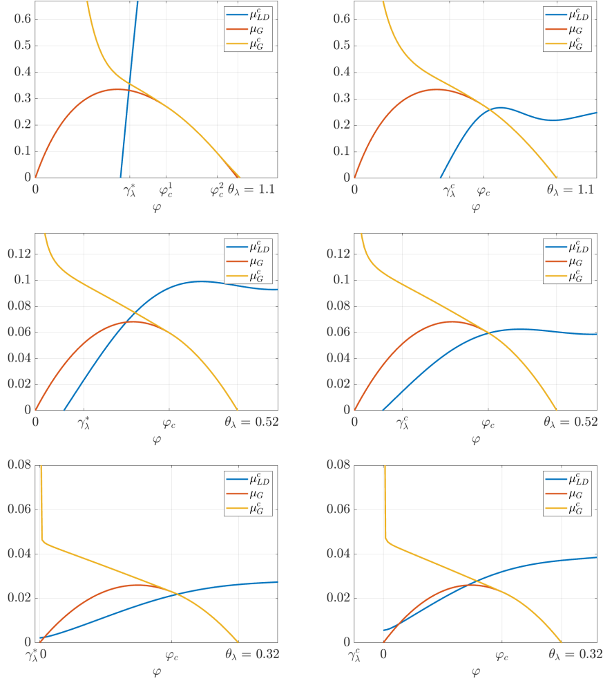
Figure 6.2: Graphs of the functions \mu_{LD}^c , \mu_G^c and \mu_G for \lambda = 0.5 (top), \lambda = 1.75 (middle), \lambda = 3 (bottom). Left: (\gamma_\lambda, c_\lambda) = (\gamma_\lambda^*, c_\lambda^*) , right: (\gamma_\lambda, c_\lambda) = (\gamma_\lambda^c, c_\lambda^c) . The values of these parameters are given in Table 6.1. Note that these figures are similar to the scheme given in [22, Figure 3.27, p.126].
