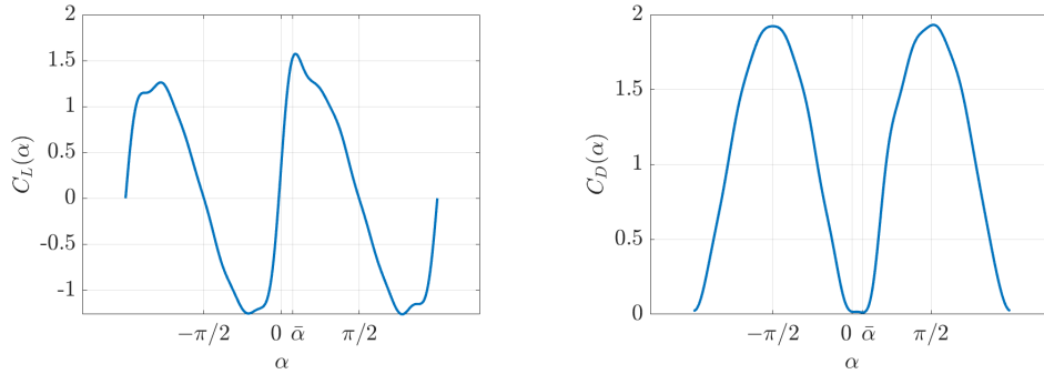
Figure 6.1: Lift and Drag coefficients C_L and C_D as functions of the angle of attack \alpha .
