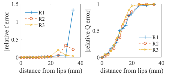
Figure 2: Relative error made on resonance frequencies and quality-factor measurements with cylinder inlet distance.
