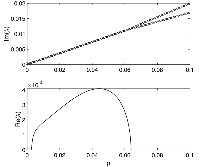
Fig. 4. Radian frequency (top) and rate of growth (bottom) of the normal mode perturbation against its wavenumber for \Omega = 0 and ak = 0.20 .
