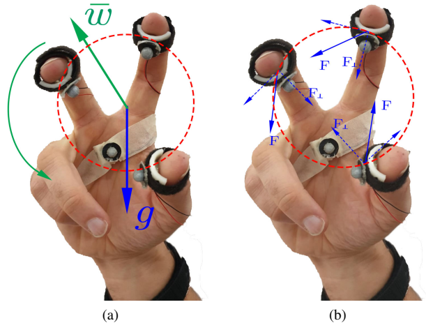
Fig. 2: Users are tasked to rotate the hand aligning the wrench \bar{\mathbf{w}} generated by the virtual object (red dashed circle) with the gravity g . The contact points position (b) is estimated using a high precision tracking system. We tested two situations in which three and four contact points are involved in the grasp. For each scenario, four different modalities were evaluated: i ) contact force and variable intensity (F+V); ii ) normal contact force component and variable intensity ( F_{\perp} +V); iii ) contact force and constant intensity (F+C); iv ) normal contact force component and constant intensity ( F_{\perp} +C).
