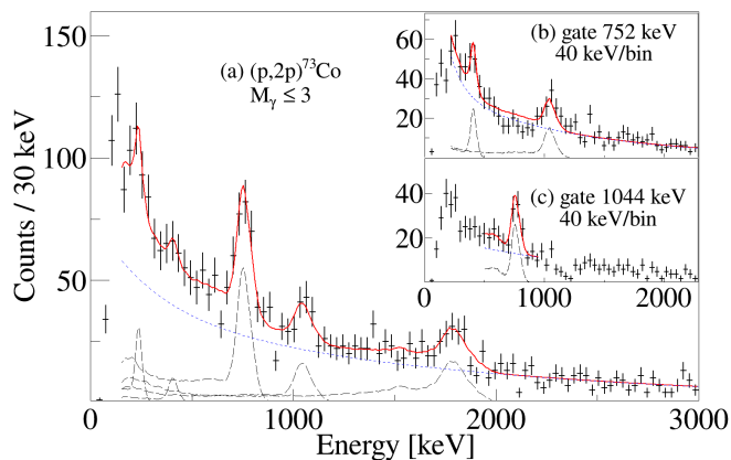
FIG. 5. (Color online) (a) Doppler-corrected \gamma -ray spectrum for ^{73}\text{Co} populated via the (p, 2p) reaction. \gamma - \gamma coincidence spectra are shown as insets without background subtraction and all M_\gamma , a gate on 752-keV, (b), and a gate on 1044-keV (c). Individual response functions for each transition are shown as long-dashed black curves, background as short-dashed red curves, and data fits as solid red curves.
