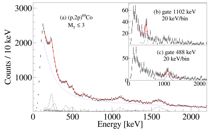
FIG. 3. (Color online) (a) Doppler-corrected \gamma ray spectrum for ^{69}\text{Co} populated via the ^{70}\text{Ni}(p, 2p)^{69}\text{Co} reaction. \gamma - \gamma coincidence spectra for the ( p, 2p ) reaction are shown in the insets with a gate on the 1102-keV transition, (b), and a gate on the 488-keV transition, (c). The analysis was made for \gamma ray multiplicity, M_\gamma = 2 for (b) and M_\gamma \leq 3 for (c). Individual response functions for each transition are shown as long-dashed black curves, background with short-dashed red curves, and data fits with solid red curves.
