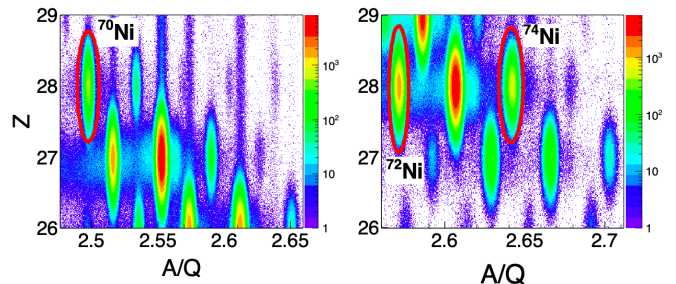
FIG. 1. (Color online) Particle identification plot for radioactive ions passing BigRIPS for the first (left) and second setting (right).
