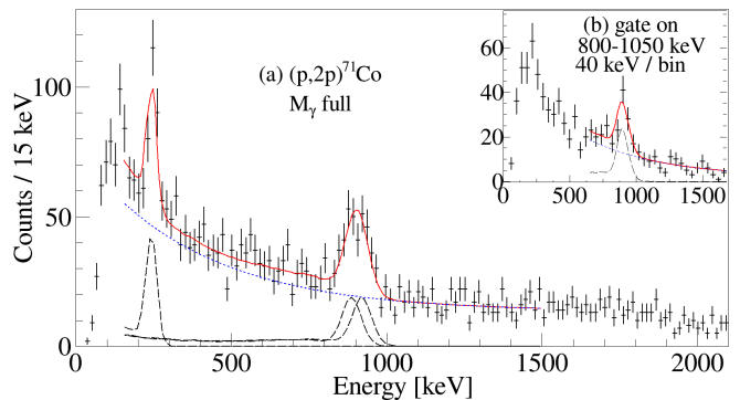
FIG. 4. (Color online) (a) Doppler-corrected \gamma -ray spectrum for ^{71}\text{Co} populated via the ( p, 2p ) reaction. Inset (b) shows the \gamma - \gamma coincidence spectrum with a gate on the 800 – 1050 keV region and considering all M_\gamma (background is not subtracted). Individual response functions for each transition are shown as long-dashed black curves, background as short-dashed red curves, and data fits as solid red curves.
