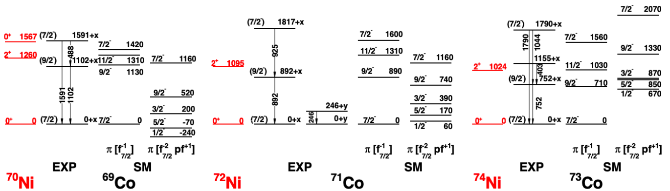
FIG. 6. Proposed level schemes and tentative spin-parity assignments for ^{69,71,73}\text{Co} and according shell model calculations using the LNPS and PFSDG-U interactions. The relative position of spherical and deformed states was not measured during the experiment. The relative position of decay bands is defined with respect to “x” and “y” shifts, which can take on different values for each level scheme. Values of 0^+ and 2^+ Ni states are taken from Ref. [36, 47] See text for details.
