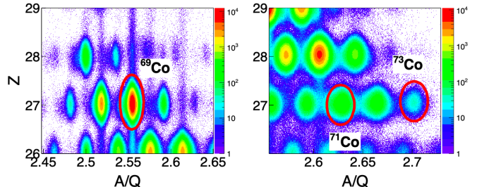
FIG. 2. (Color online) Particle identification plot for radioactive ions arriving at ZeroDegree for the first (left) and second setting (right).
