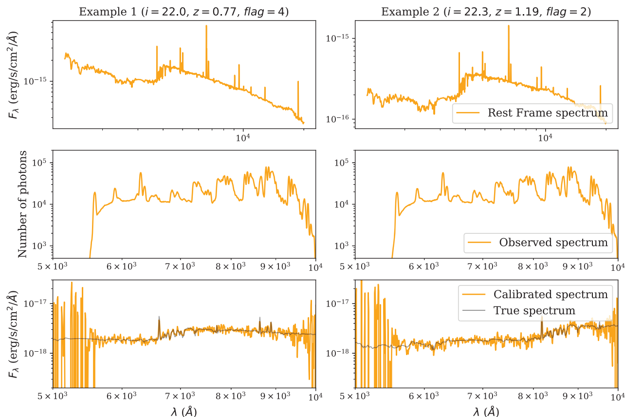
Figure 1. Example spectra from the simulated VVDS Deep survey. Top panels: Original rest-frame linear combination of k -correct components. Middle panels: Poisson-sampled spectrum including sky emission. Note that the apparent shape of the spectrum is dominated by the sky emission. Bottom panels: Final sky-subtracted and calibrated simulated spectrum (yellow) overlaid with the true spectrum (black). The former is what is passed on to the next stage for redshifting. The i -band magnitudes as well as the true redshifts for the two galaxies are listed at the top of the figure. The spectra on the left represent an example of a good spectrum (Flag = 4), while the spectra on the right represent a spectrum of relatively poor quality (Flag = 2).
