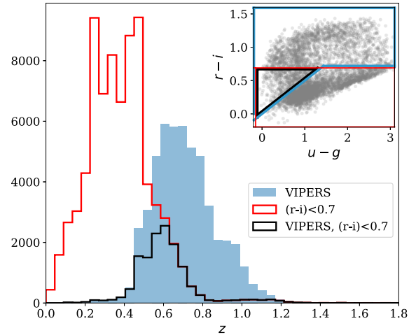
Figure 4. Redshift distribution of galaxies matching the VIPERS colour selection: (r - i) > 0.5(u - g) or (r - i) > 0.7 (solid), an (r - i) < 0.7 sample, and a sample selecting just where VIPERS overlaps at (r - i) < 0.7 . These latter two samples have different redshift distributions, and so re-weighting without (u - g) colour information will result in biases. Inset: these three samples in (u - g) versus (r - i) colour space.
