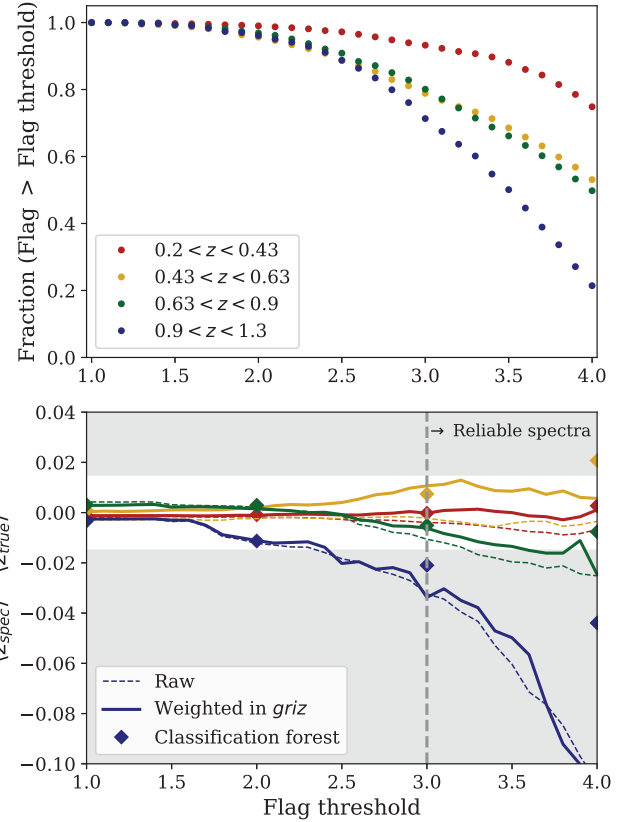
Figure B1. Same as the top two panels of Fig. 6, but for VVDS Deep (field 1) alone.
