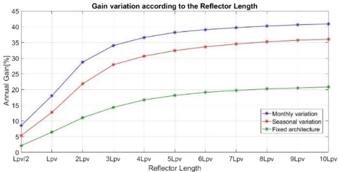
Fig. 9. G_A variation according to the reflector's length for a monthly varied, seasonal varied and a fixed architecture.
