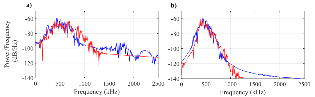
Figure 3. Power spectral density (PSD) of (a) the unfiltered “reference” waveform obtained at the receiver from the simulation (blue line) and measured in the laboratory experiments (red line) with an unstressed sample, (b) after filtering in the (300–600) kHz frequency band.
