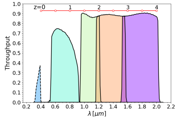
Figure 1. Throughput of the four main Euclid filters (coloured regions and solid black lines). From the left- to right-hand side, these are the VIS filter, and the NISP/Y , NISP/J , and NISP/H filters. We also include the throughput of the CFIS/u -band filter (blue region, dashed black line). The red dots indicate the observed wavelength of the 4000-Å break at different redshifts.
