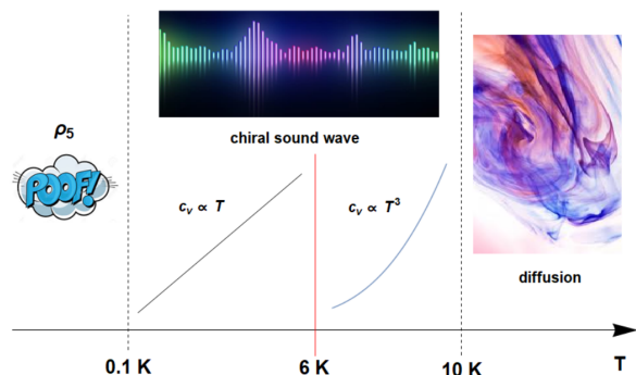
FIG. 1: Fate of the chiral sound and behavior of the specific heat discussed in the text. For T < 0.1 \text{ K} the internode life time is too short and the chiral sound wave would not propagate. A linear behavior of the specific heat will prevail in the range 0.1 \text{ K} < T < 6 \text{ K} and the T^3 phonon contribution takes over at T > 6 \text{ K} . For T > 10 \text{ K} the chiral wave will be diffusive.
