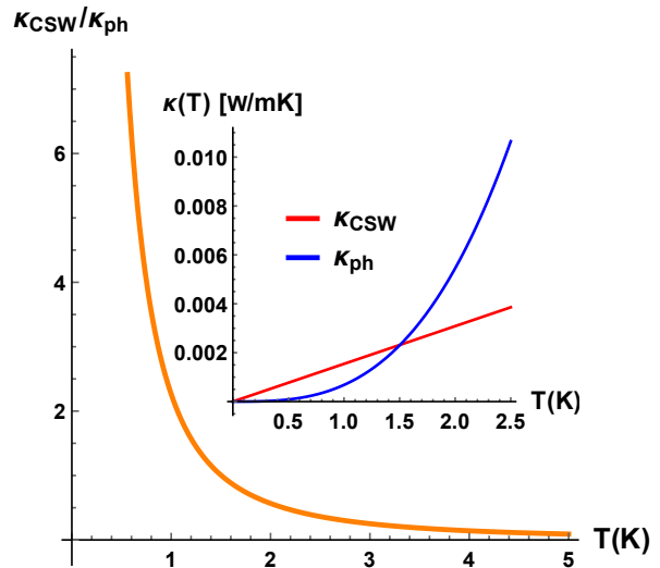
FIG. 2: Rate of the CSW and the acoustic phonon contribution to the longitudinal thermal conductivities along the axis of the twist. The two contributions are shown in the inset. At temperatures below 1.5 K the CSW contribution is dominant.
