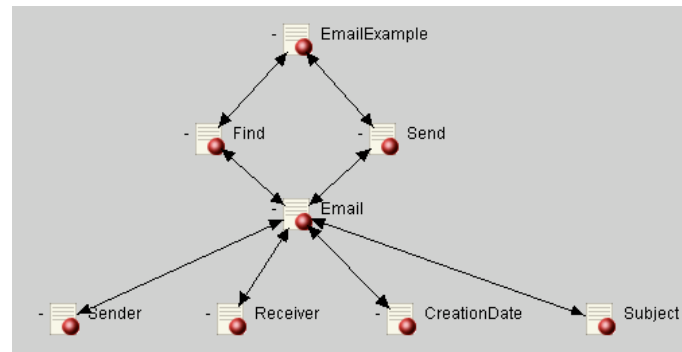
Fig. 5. An example AAOSA agent network
