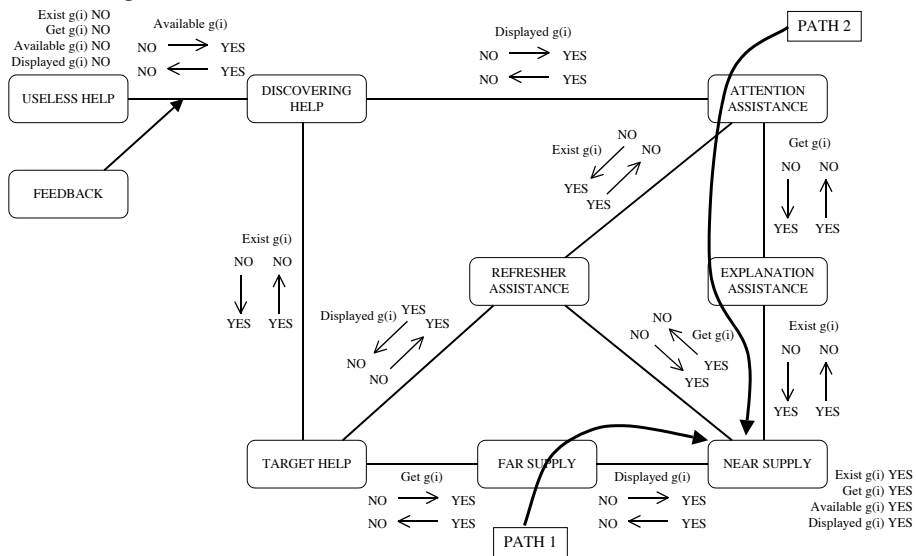
Fig. 2. Documentation activities workload categories paths
