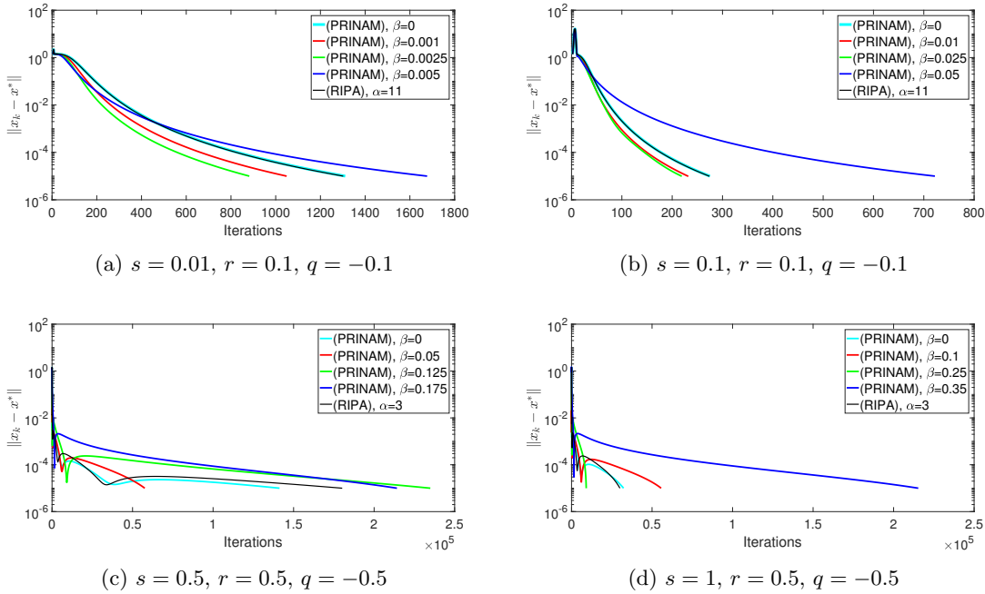
Fig. 1.2: Iteration error \|x_k - x^*\| for different instances of (PRINAM) and (RIPA)
