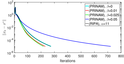
(b) s = 0.1 , r = 0.1 , q = -0.1
