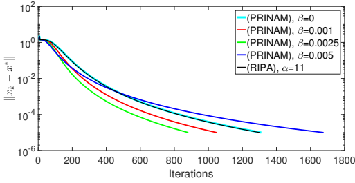
(a) s = 0.01 , r = 0.1 , q = -0.1
