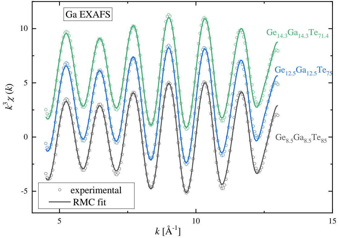
Figure 4. k^3 -weighted, filtered EXAFS spectra at Ga K-edge (symbols) and fits (lines) of the Ge_xGa_xTe_{100-2x} glasses. (The curves are shifted vertically for clarity.)
