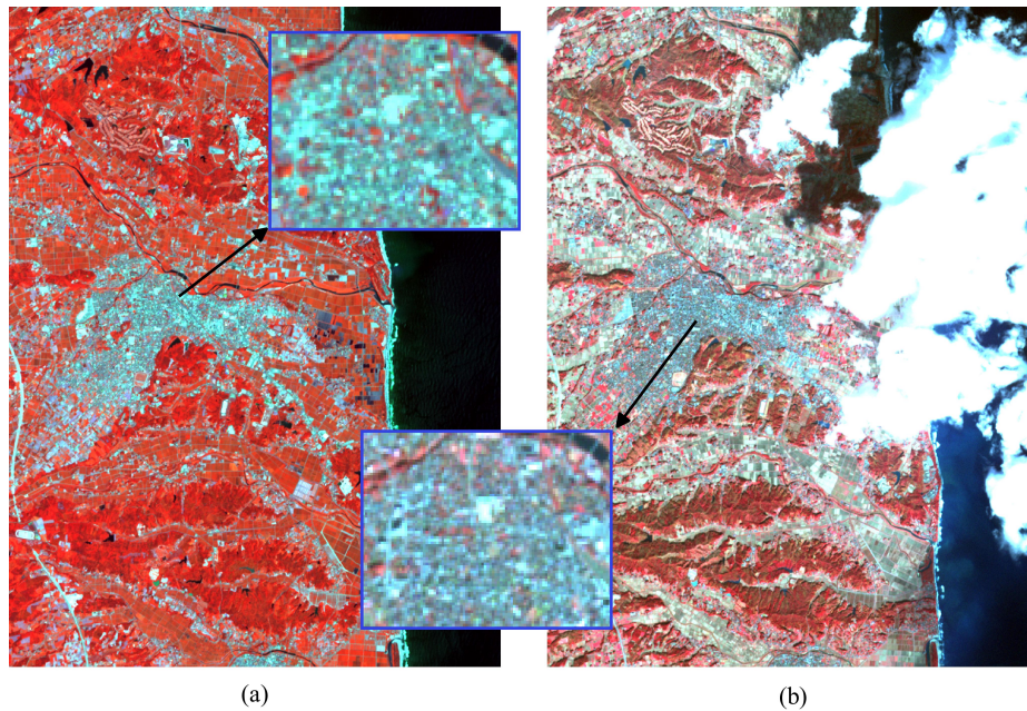
Figure 1. Two ASTER images taken on (a) July 2010 and (b) November 2010. Image (a) was taken in sunny conditions that caused much higher pixel values for urban area pixels (zoomed) than for image (b). For example, the value of the same pixel of this area is equal (83, 185, 126) for (a) and (37, 63, 81) for (b). Moreover, a great part of image (b) is covered by clouds and their shadow.
