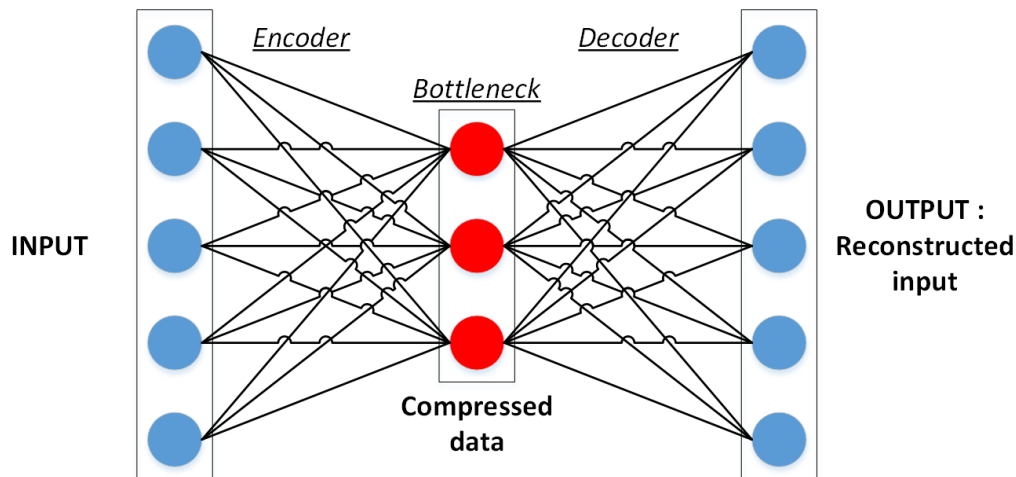
Figure 3. Basic architecture of a single layer autoencoder made of an encoder going from the input layer to the bottleneck and the decoder from the bottleneck to the output layers.
