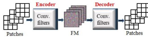
Figure 5. Fully convolutional AE model.
