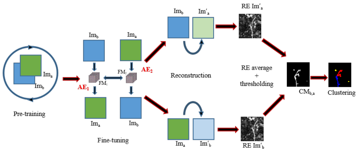
Figure 4. Algorithm flowchart.
