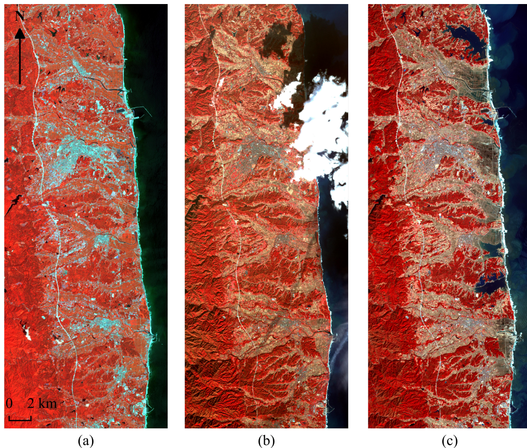
Figure 6. Images taken over the damaged area, (a) 7 July 2010, (b) 29 November 2010, (c) 19 March 2011.
