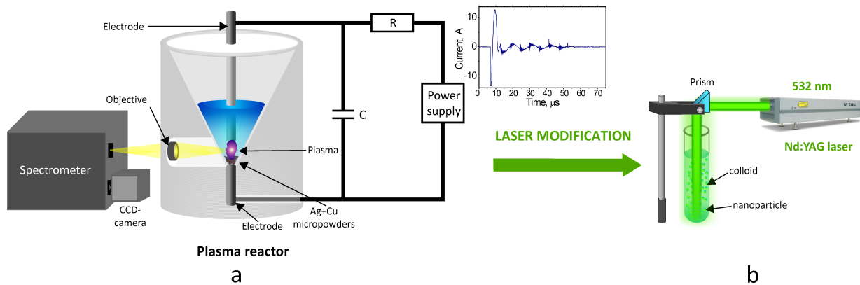
Figure 1. Scheme of the two-step process with a 5 min plasma treatment (a) followed by a 5 min laser treatment (b)
