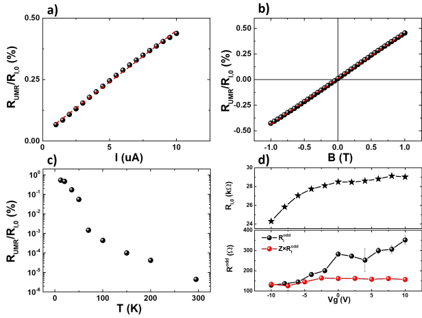
Figure 3. (color online) R_{\text{UMR}} normalized to the zero magnetic field resistance R_{l,0} taken at \varphi = 270^\circ (in %) as a function of (a) the applied current for B = 1 T and T = 15 K (b) the magnetic field for I = 10 \mu\text{A} and T = 15 K, and (c) the temperature for B = 1 T and I = 10 \mu\text{A} . Red dotted lines are linear fits. (d) Gate voltage dependence of R_{l,0} , R_{t,\text{max}}^{\text{odd}} and ZR_{t,\text{max}}^{\text{odd}} , R_{\text{UMR}} = R_{l,\text{max}}^{\text{odd}} - ZR_{t,\text{max}}^{\text{odd}} .
