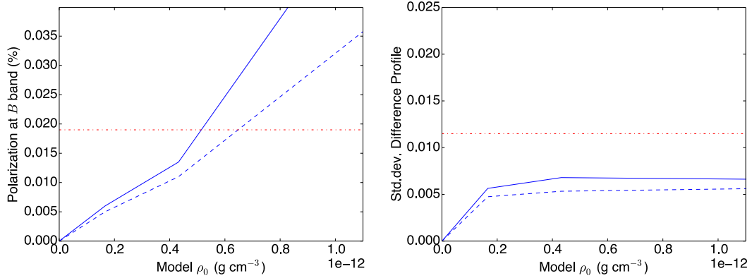
Fig. 4. Polarization in the B band (left) and standard deviation of difference H \alpha profile (right) as a function of disk-base density \rho_0 for the residual disk models from Table 5 (model 1: full line; model 2: dashed line). The standard deviation is the root mean square of the disk model spectrum minus the pure photospheric profile. The horizontal dot-dashed lines represent the observational limits of average polarization and difference profile determined from observations performed at the epoch of interferometric observations, as explained in Sect. 3. While the measured H \alpha difference profile level does not impose a limit to \rho_0 , the measured average polarization sets a strict upper limit to this quantity: \rho_0 < 0.52 \times 10^{-12} \text{ g cm}^{-3} for the thin-disk model and \rho_0 < 0.65 \times 10^{-12} \text{ g cm}^{-3} for the thick-disk model.
