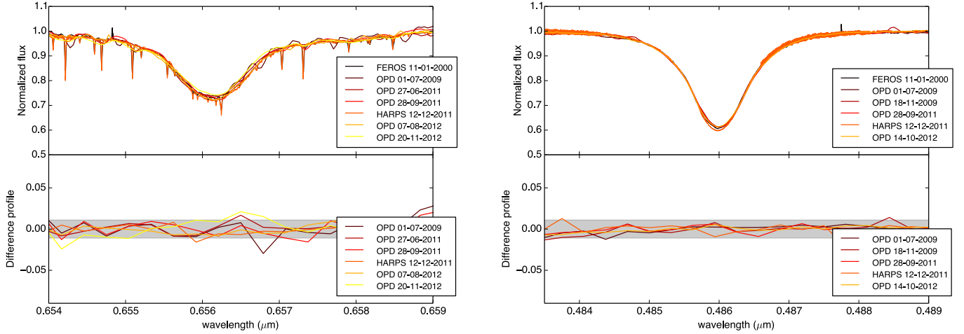
Fig. 3. Top: H \alpha (left) and H \beta (right) line profiles of Achernar at the epoch of interferometric observations. Bottom: difference in flux of the line profiles with respect to the reference FEROS spectrum from 2000 Jan. 11. This spectrum can be considered as a good approximation to the pure photospheric profile of Achernar (Rivinius et al. 2013). Whenever possible (enough spectral resolution) the telluric lines seen in some spectra have been removed before computing the differences. The horizontal shaded (gray) areas indicate the typical error on the difference profiles and also set a limit to them.
