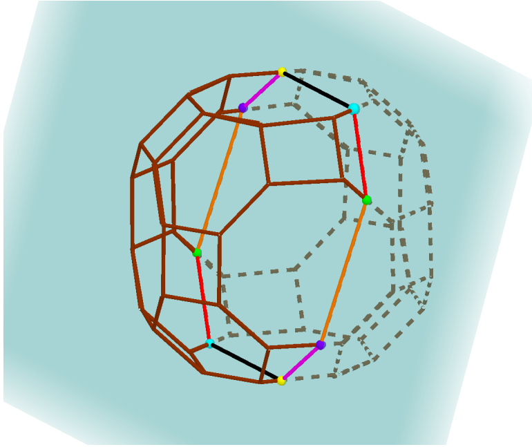
Figure 4: Illustration of the signed permutahedron P_w^\pm (in brown) and the plane \text{row}(X) (in light blue). Because \text{rk}(X) = 2 and \text{row}(X) does not intersect any vertex of P_w^\pm (the faces with codimension equal to 3), the SLOPE estimator \hat{\beta}_w(y) is unique for all values of y \in \mathbb{R}^2 . Colored segments and points are the intersections between \text{row}(X) and the faces of P_w^\pm , determining the accessible SLOPE patterns shown in Table 1. For example, m = (2, 1, 1)' is an accessible SLOPE pattern, which implies that there exists y \in \mathbb{R}^2 for which the SLOPE minimizer \hat{\beta}_w(y) satisfies \hat{\beta}_w(y)_1 > \hat{\beta}_w(y)_2 = \hat{\beta}_w(y)_3 > 0 . In addition, since m = (2, 1, 0)' is not an accessible pattern, one cannot pick y \in \mathbb{R}^2 for which the SLOPE minimizer satisfies \hat{\beta}_w(y)_1 > \hat{\beta}_w(y)_2 > \hat{\beta}_w(y)_3 = 0 .
