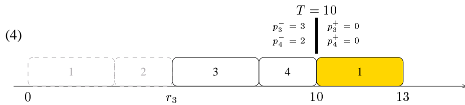
Figure 4: The first steps of SN
