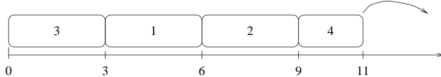
Figure 5: An optimal schedule for the non-preemptive problem with release dates.
