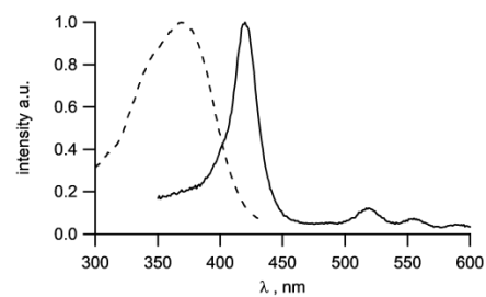
Fig. 3. Emission and excitation spectra of the FONPs[TPP] . A: emission spectra (dotted line, \lambda_{ex} = 360 nm and solid line, \lambda_{ex} = 520 nm); B: excitation spectra (dotted line, \lambda_{em} = 450 nm and solid line, \lambda_{em} = 650 nm)
