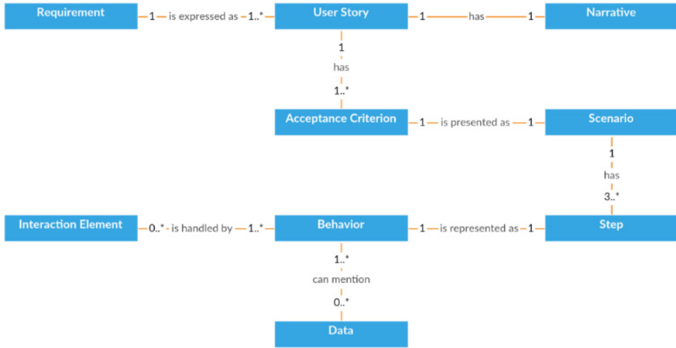
Fig. 2. Conceptual model of user requirements.
