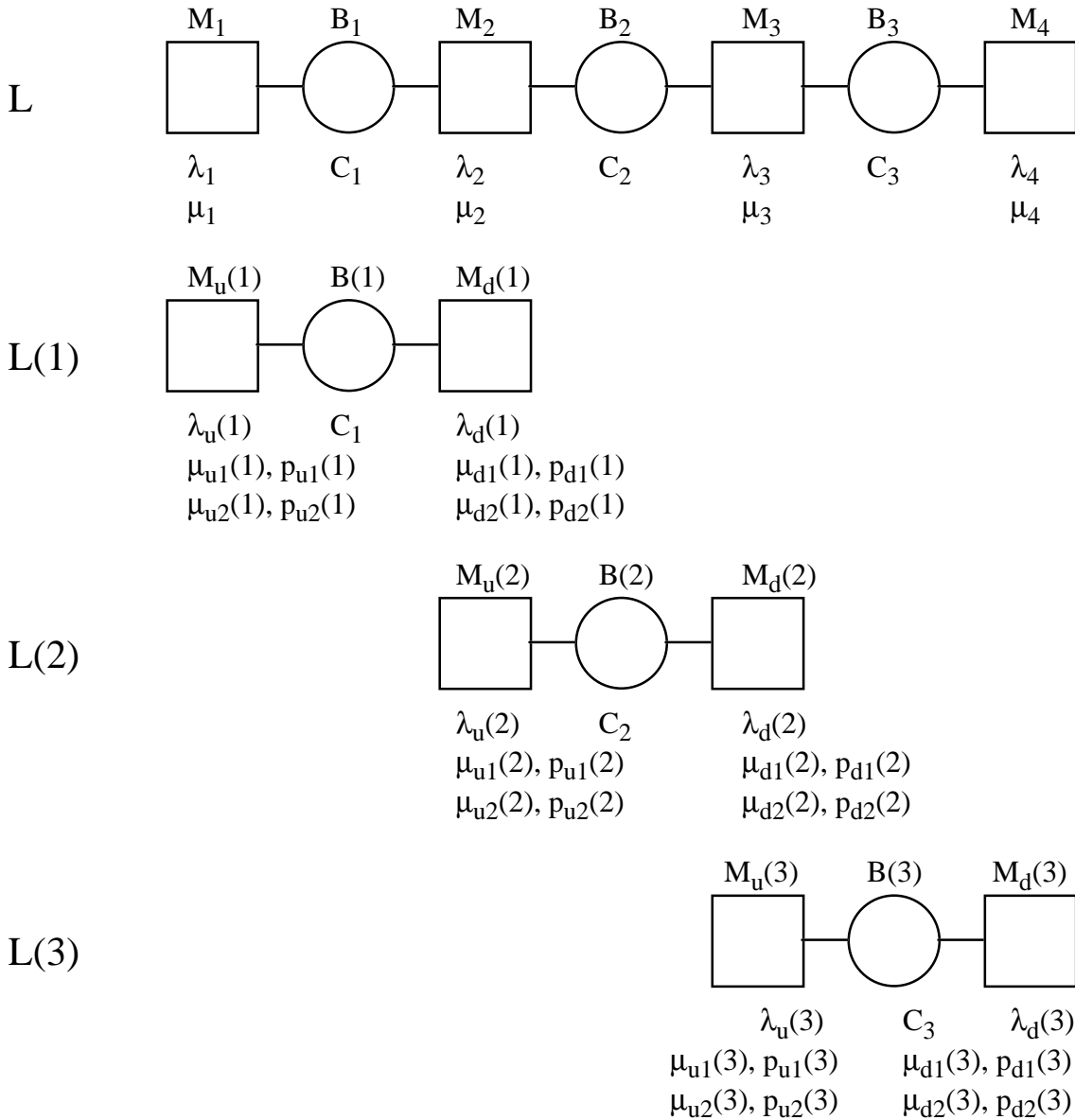
Figure 1: A four-machine production line and its decomposition into three two-machine production lines.
