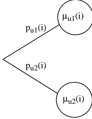
Figure 3: Illustration of the two-stage hyper-exponential approximation of the repair time distribution of machine M_u(i) .
