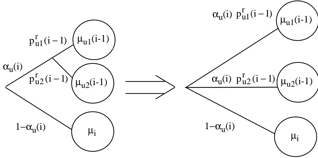
Figure 4: Illustration of the construction of the repair time distribution of machine M_u(i) .
