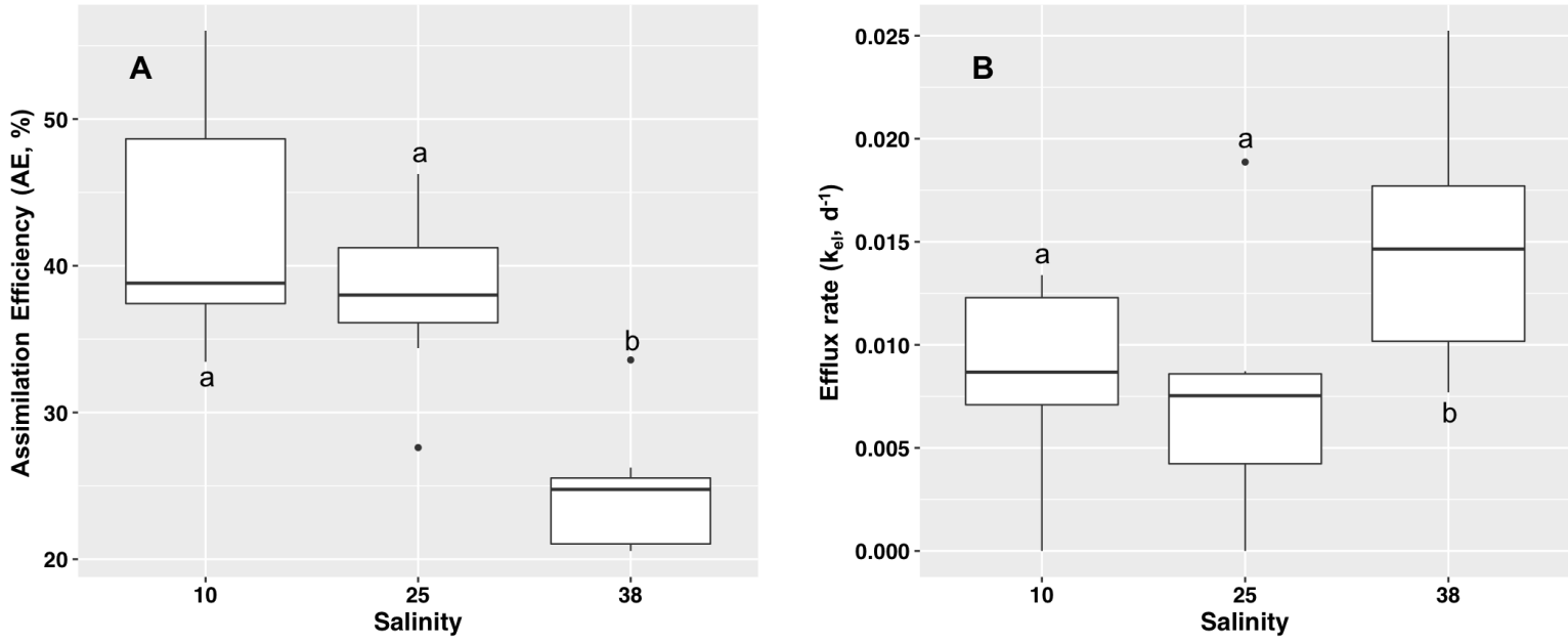
Figure 2. Comparison of (A) assimilation efficiencies (AEs) and (B) efflux rate constant ( k_{ei} ) of Mn calculated for each individual turbot acclimated to three salinity conditions. The best fitting model obtained for the entire set of turbots (see Fig. 1 and Table 2) was applied to individuals. Letters denote significant differences between the salinity conditions.
