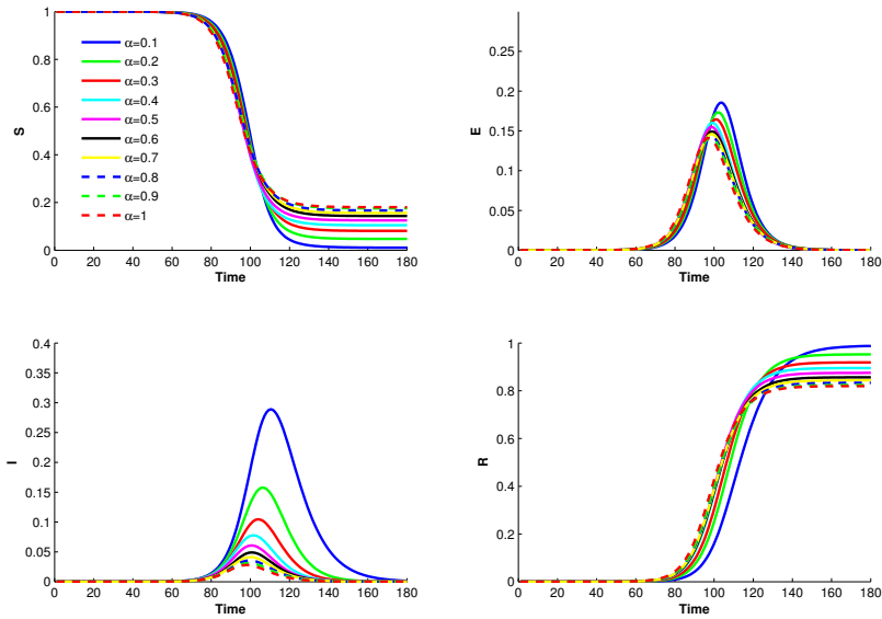
FIGURE 4. Impact of the average time in compartment I before isolation on the solutions of SEIR system (2)-(6).
