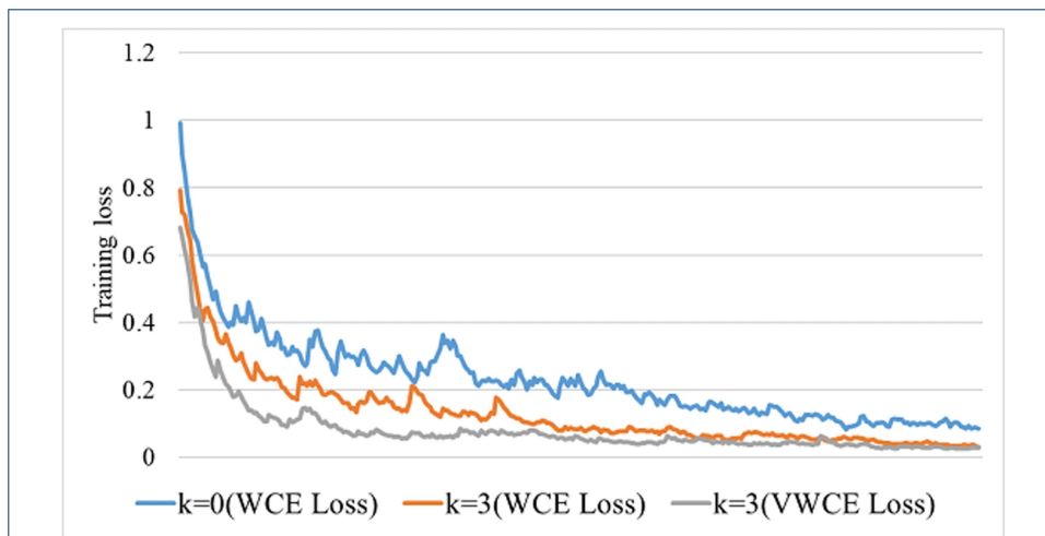
Figure 6 Training losses of the final CNN model in stage3 with different parameters
