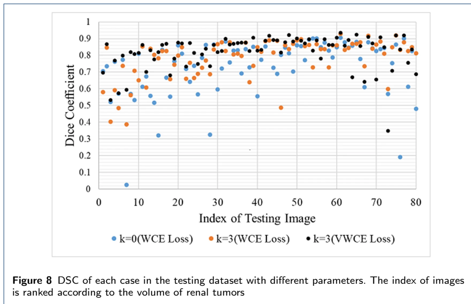
Figure 8 DSC of each case in the testing dataset with different parameters. The index of images is ranked according to the volume of renal tumors
