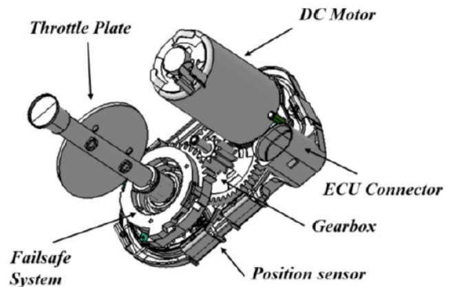
Fig. 2: Electronic Throttle Body architecture.
