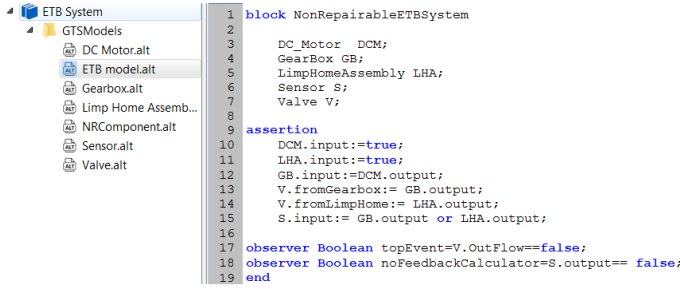
Fig. 5: Safety analysis of the ETB (Altarica).
