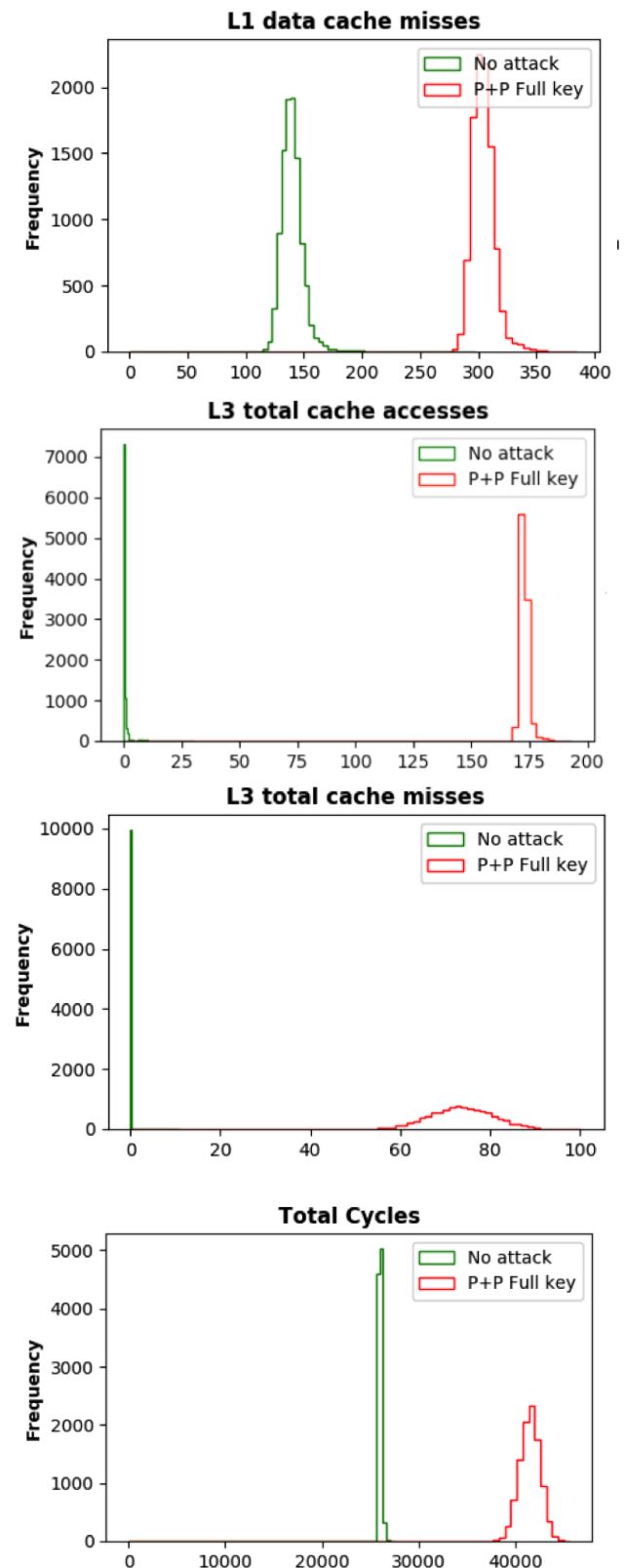
FIGURE 2: Results showing selected hardware events under no load condition for Prime+Probe attack on AES.
