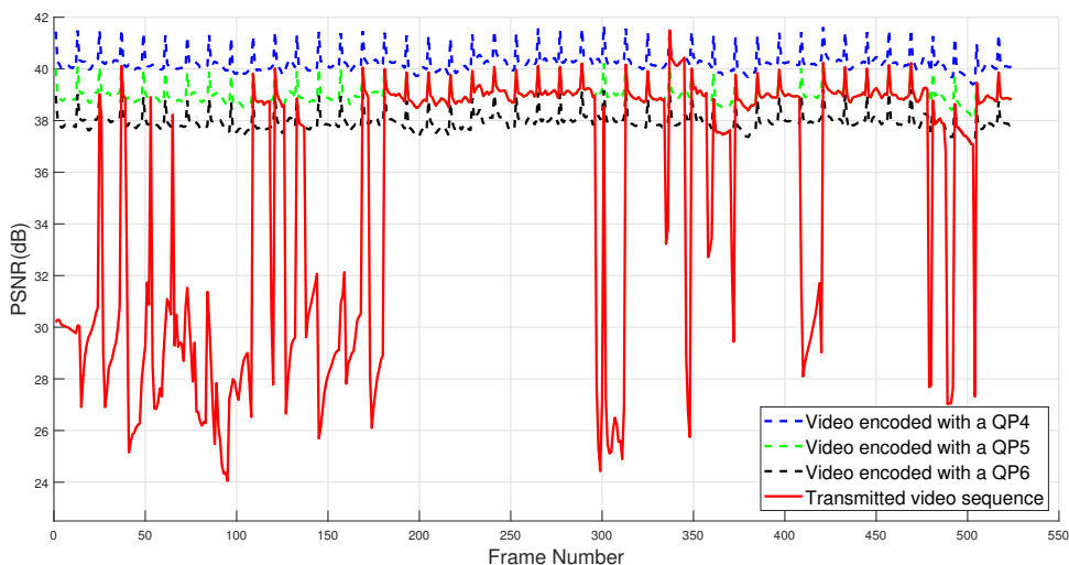
Figure 1: PSNR variation for adaptive video transmission.
