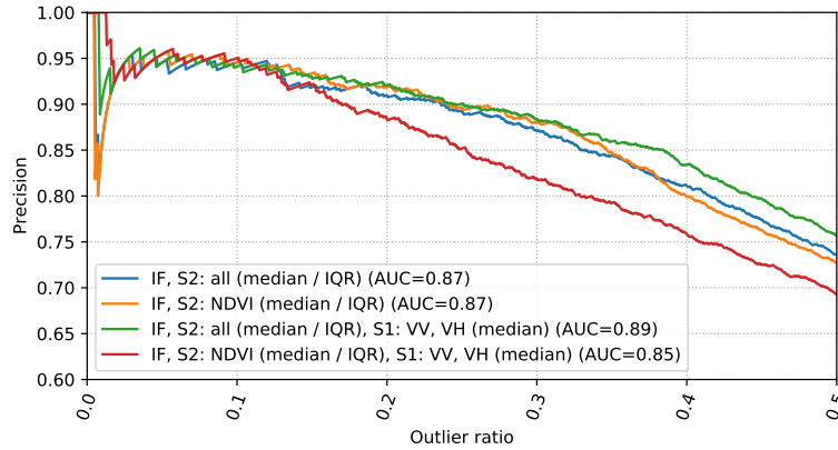
Fig. 13: Precision vs. outlier ratio for a complete growing season analysis of the rapeseed parcels. Various sets of features using the IF algorithm are compared.
