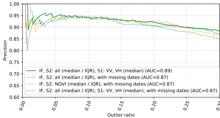
Fig. 19: Precision vs. outlier ratio for a complete season analysis of the rapeseed dataset. Missing dates means that only 1 S2 images out of 2 was taken (6 S2 images instead of 13).
