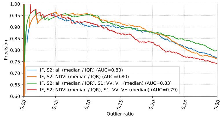
Fig. 21: Precision vs. outlier ratio for a mid-season analysis of rapeseed parcels (all images available before February). Various sets of features are compared using the IF algorithm.
