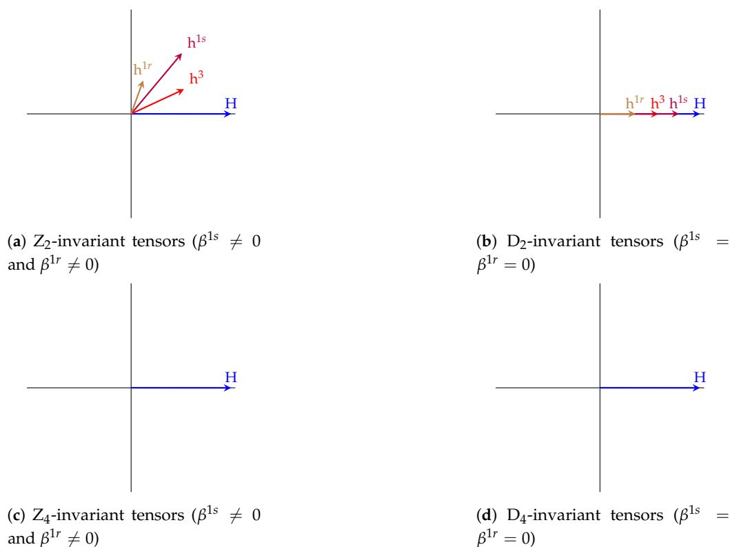
Figure 2. Representation of flexoelectric tensors using harmonic tensors (the hemitropic and isotropic coefficients are not represented here).
