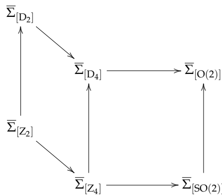
Figure 1. Bifurcation diagram of Flex.
