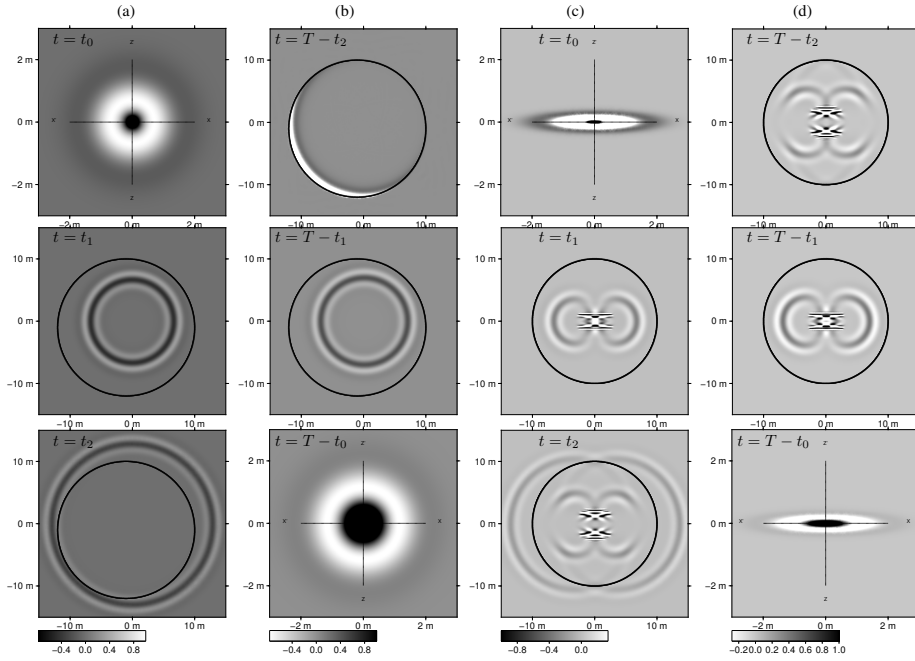
Figure 3: Pressure field snapshots at different time steps for the forward modeling step in a homogeneous medium (a), for the corresponding backward step (b), for the forward step in the anisotropic medium (c) and for the corresponding backward step (d). t = t_0 is the source origin time for the forward modeling sequences (a) and (c). t = T - t_0 corresponds to the focusing time for the backward modeling sequences (b) and (d). For the homogeneous case t_0 = 0.02s , t_1 = 0.04s , t_2 = 0.058s and T = 0.1s . For the anisotropy case, t_0 = 0.01s , t_1 = 0.03s , t_2 = 0.05s and T = 1.0s . Note that panels don't have all the same spatial scale. The TRM circle has deliberately not been centered on the source for the left plots (a) and (b): it shows that the position of the TRM with respect to the source is irrelevant to its capacity to focus the wavefield back to the source location.
