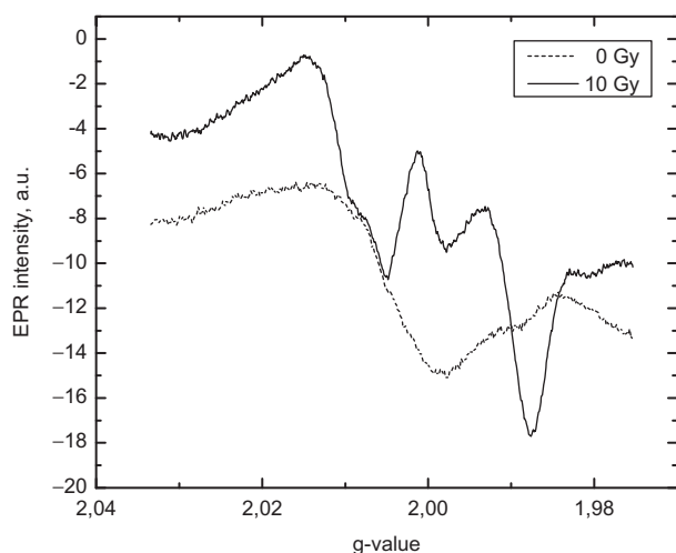
Figure 2. Electron Paramagnetic Resonance (EPR) spectra of unexposed and 10 Gy exposed Gorilla Glass ® samples.
