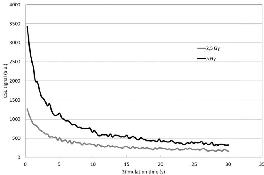
Figure 1. Example of Optically Stimulated Luminescence (OSL) curve for resistors irradiated respectively at 2.5 and 5 Gy.
