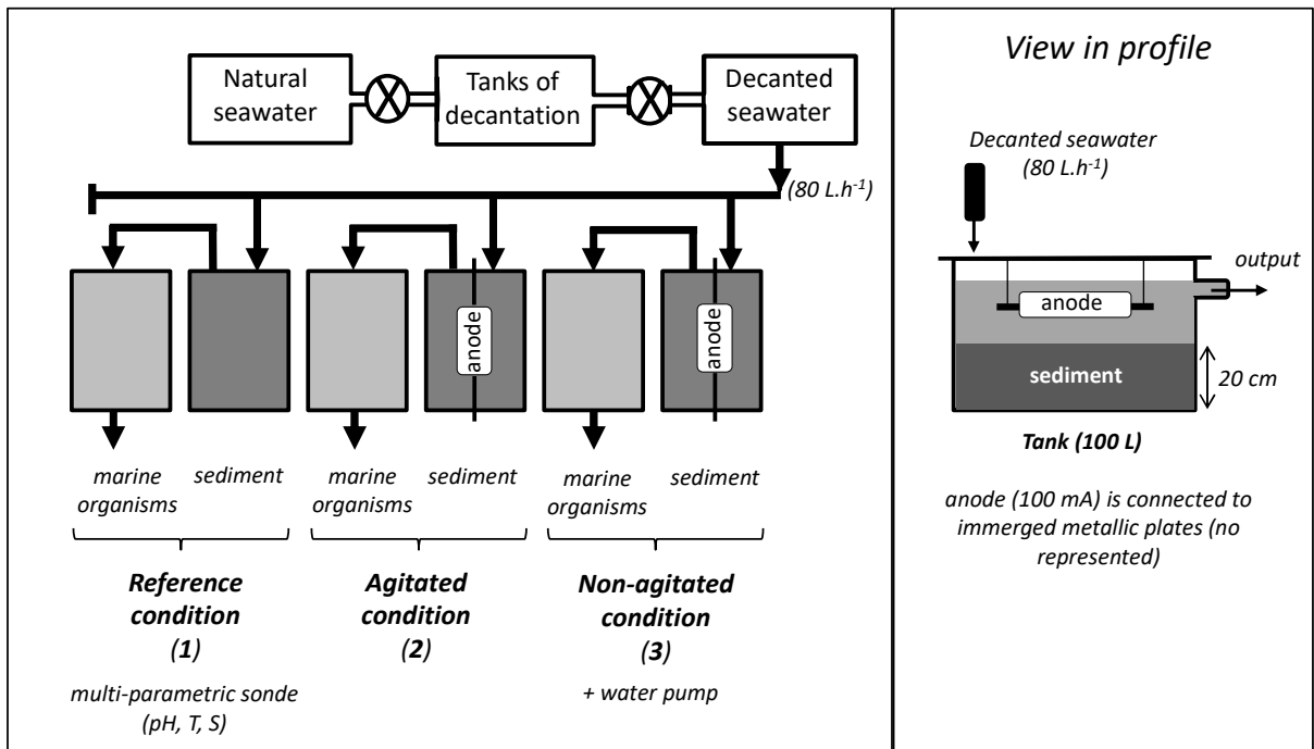
170 Fig. 2: Experimental devices with or without a galvanic anode to reproduce anode degradation under laboratory 171 conditions.
