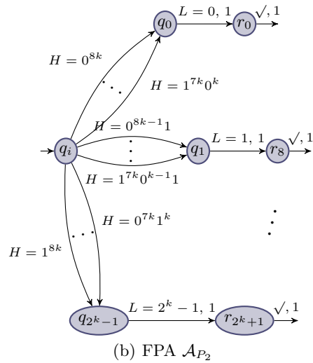
Fig. 13. FPAs for programs P_1 and P_2 .
