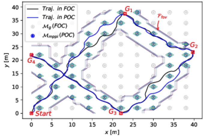
Fig. 6. The 40 m obstacle field map, i.e., 2D \mathcal{M}_g , and its updated 2D \mathcal{M}_{mppi} map using a 5 \times 5 2D \mathcal{F}_{fov} . Two lines represent the trajectories generated by MPPI in both cases, i.e., FOC and POC .
