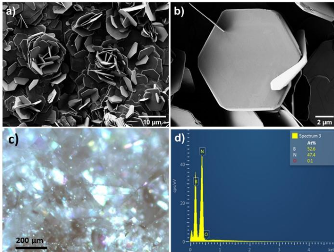
Figure 3. a,b) Low resolution SEM micrographs of the h-BN sample located on the top inner surface of the crucible. In a) faceted flower-like crystals are observed and b) shows the detail of one h-BN crystal. Corresponding c) optical image and d) EDS spectrum recorded using SEM.
