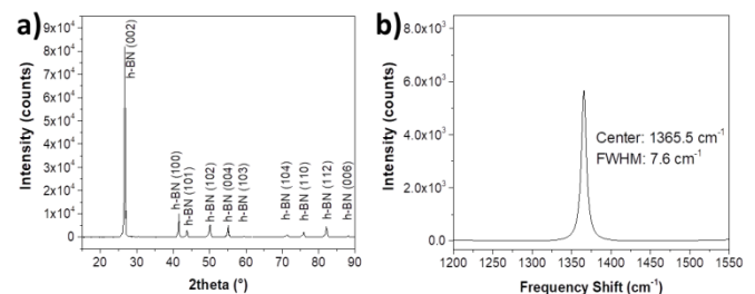
Figure 5. a) XRD pattern and b) Raman spectrum of h-BN samples obtained by PDCs coupled with GPS. The peaks are indexed to the corresponding crystallographic planes in a) and the position and FWHM of the h-BN E_{2g} band are underlined in b).
