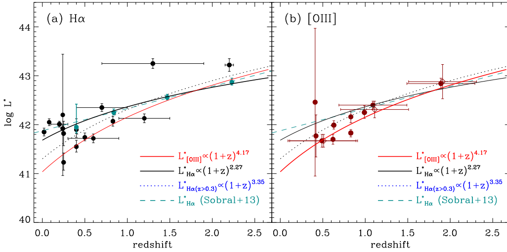
FIG. 12.— Redshift evolution of the critical value L^* of emission line luminosity functions of (a) H\alpha , and (b) [O\text{ III}] . Values are compiled from the literature, and include a direct comparison with the evolution found by Sobral et al. (2013) in green (green filled circles and dashed line). Our best-fit evolution goes like (1+z)^{2.27} for H\alpha (solid black curve on panel a) and like (1+z)^{4.17} for [O\text{ III}] (solid red curve on panel b). We also fit to H\alpha at z > 0.3 (dotted line) to enable a closer comparison with the [O\text{ III}] results. In the case of [O\text{ III}] , two open diamond symbols show repeated measurements with fixed faint-end slope. Using these two points instead of their counterpart at z = 1.1 and 1.9 (slightly offset for clarity of the plotting symbols) does not noticeably change the fit.
