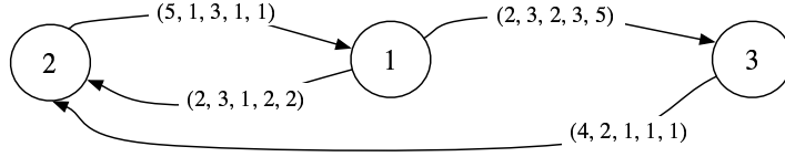
Figure 1: A linear precedence multi-graph G . Every arc a is labeled with (l_{e(a)}, p_a, p'_a, q_a, q'_a)
