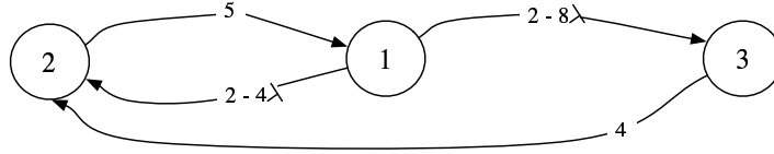
Figure 3: Graph G valued by l_a - \lambda h_a
