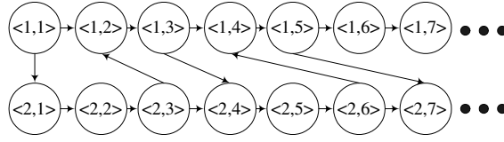
Figure 2: The developed graph of precedences
