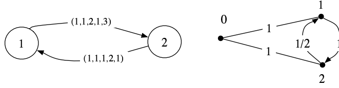
Figure 5: A linear precedence graph G and the corresponding reduced graph R
