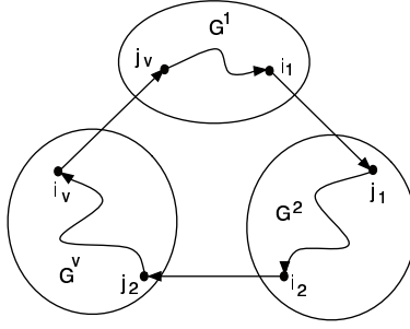
Figure 4: Definition of c
