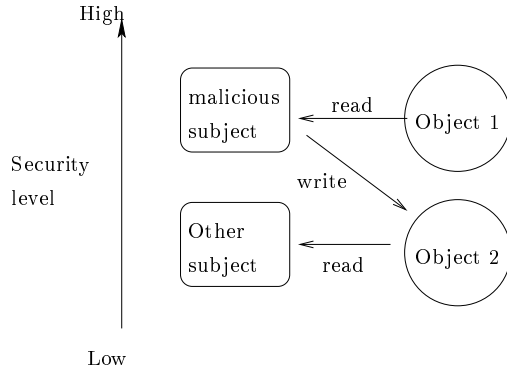
Figure 1: Violation of the \text{MAC}^* property
