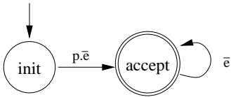
Fig. 5. Inverted Büchi automaton for Progress \Rightarrow \mathbf{F}(AllAck)
