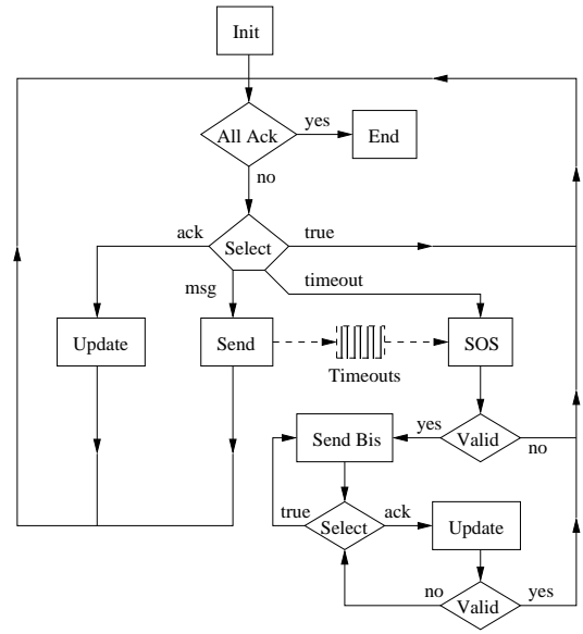
Fig. 4. the finite sequences sender's model
