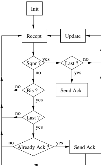
Fig. 3. the finite sequences receiver's model
