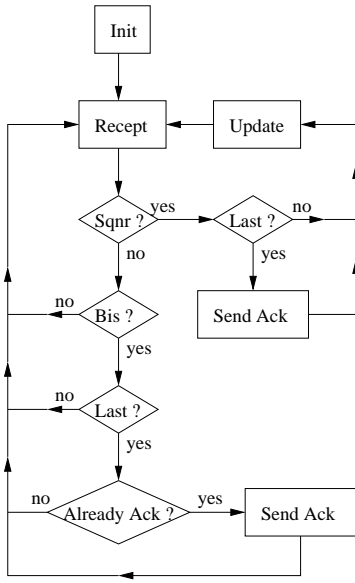
Fig. 3. the finite sequences receiver's model
