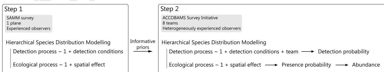
Figure 2. Methodological chart summarising the analytical procedure used for this study. We first estimated detection and presence probabilities of mega-debris in the north-western Mediterranean Sea with a Hierarchical Species Distribution Model using data from the SAMM survey, conducted in 2012. Second, we estimated detection and presence probabilities of mega-debris over the entire Mediterranean Sea from the ASI data, using parameters estimated from the SAMM survey as informative priors for the detection probability and weakly informative priors for the presence probability. Abundance estimate was eventually derived from the presence probability.
