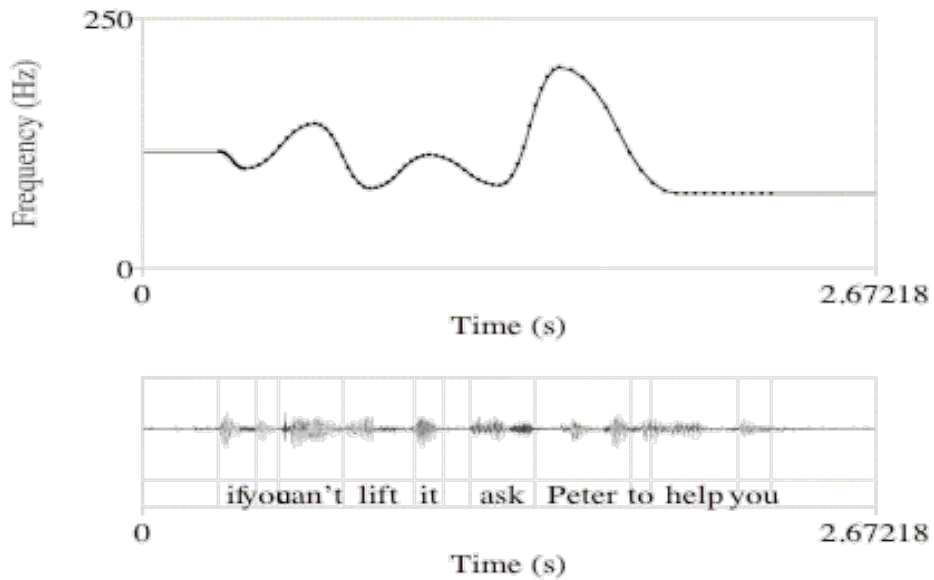
Figure 4. Continuous quadratic spline curve produced as output from the sequence of target pitches in example (6)
